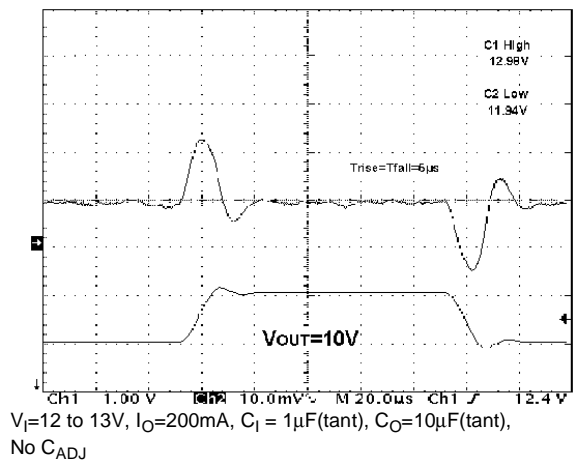
Figure 26: Line Transient
